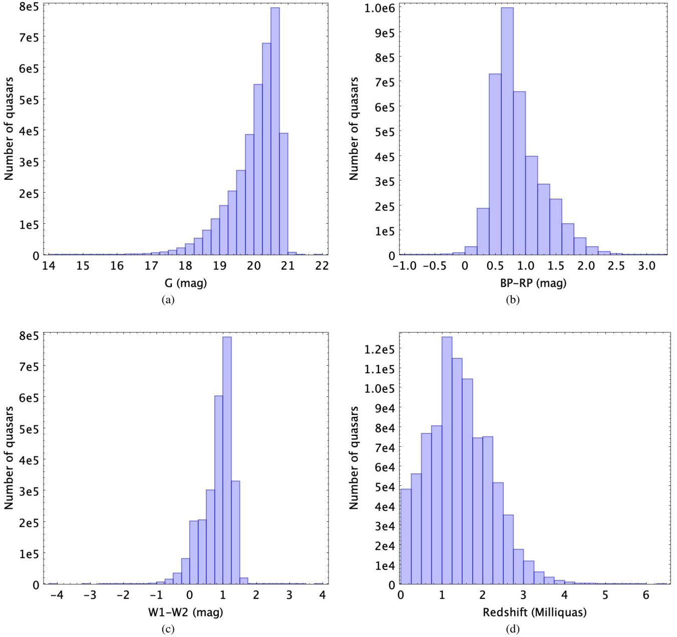
Fig. 2. Distributions of (a) Gaia G magnitudes ( phot_g_mean_mag ) from the Gaia DR3 gaia_source table, (b) G_{BP} - G_{RP} colours ( phot_bp_mean_mag - phot_rp_mean_mag ), (c) W1-W2 colours (from catWISE ), (d) redshifts (from Milliquas ) of the QSOs and candidates from the input list.
